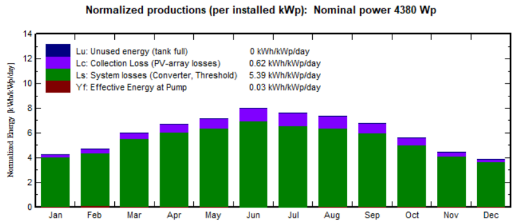
Figure 5. Solar production using PVsyst.
